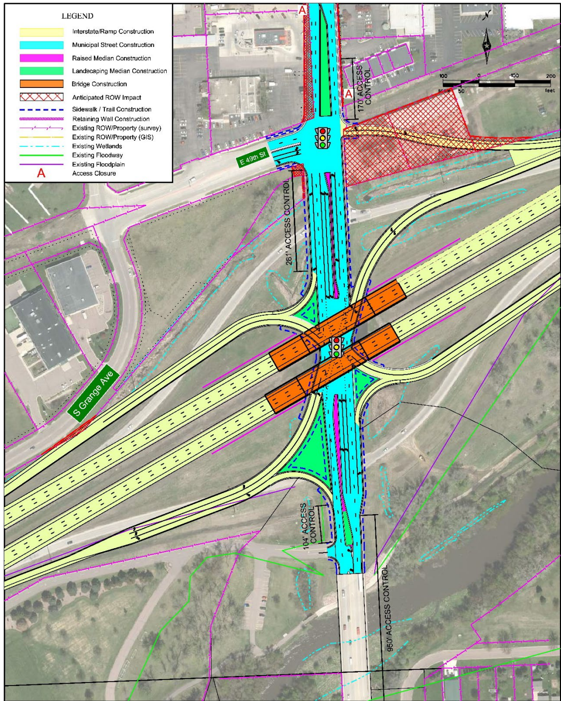
Figure 29 – Alternative 9D – Control of Access
