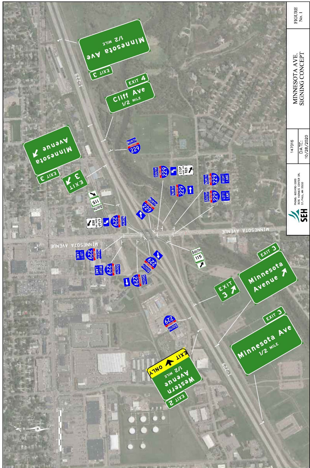
Figure 30 – Alternative 9D Conceptual Signing Plan
