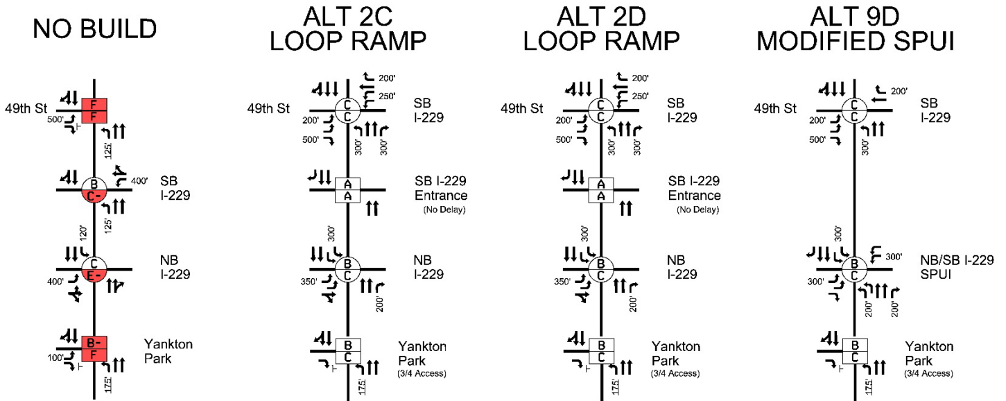
Figure 19 – 2050 Build Minnesota Avenue Interchange Configurations and LOS
